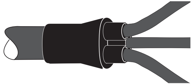
Installed 3-leg Breakout
