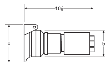
APR Connector
