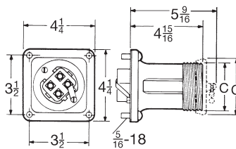
AR Receptacle - Open and With Cap
