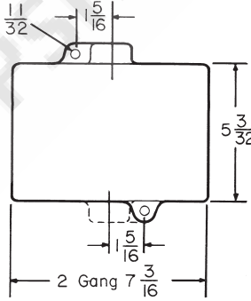
Front View - Two gang
